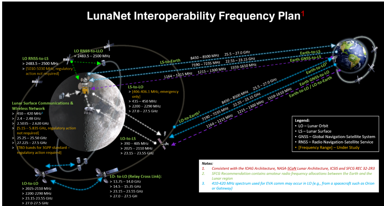
Figure 20- LunaNet Interoperability Frequency Plan
