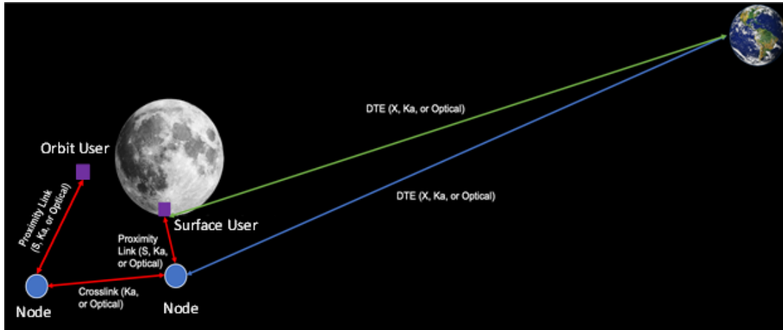
Figure 19 - Functional Interfaces and Corresponding Frequency Bands
