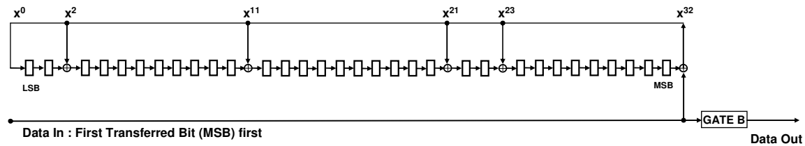
Figure 5: Improved CCSDS CRC-32 Decoder Diagram
