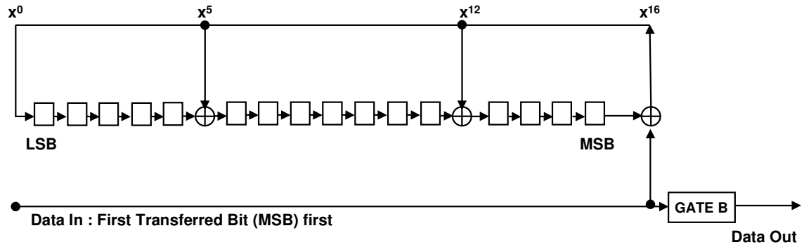
Figure 4: Improved CCSDS CRC-16 Encoder Diagram
