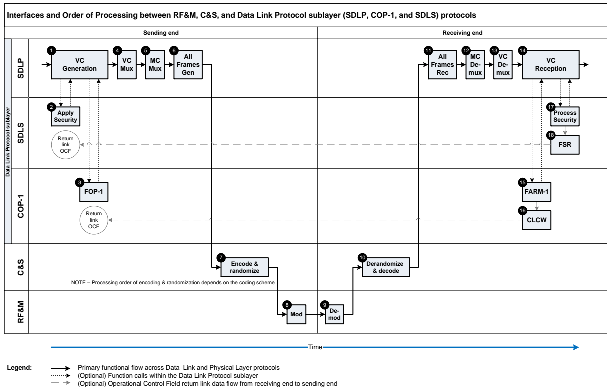
Figure 3-3: Order of Processing between TC SDL and SDLS Functions
