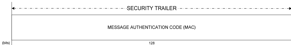
Figure A-4: Security Trailer (TM Baseline)
