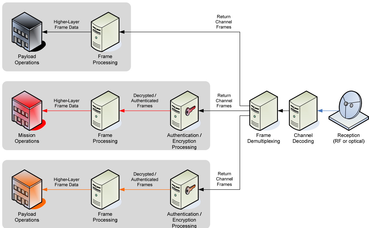
Figure 4-9: Complex Return Link Scenario (Ground)
