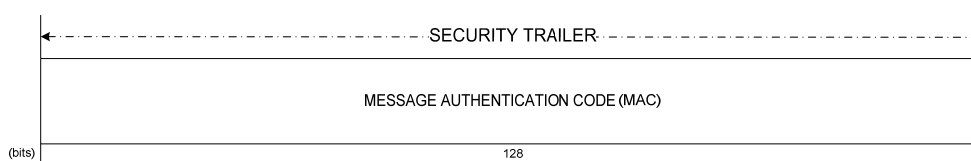
Figure A-2: Security Trailer (TC Baseline)
