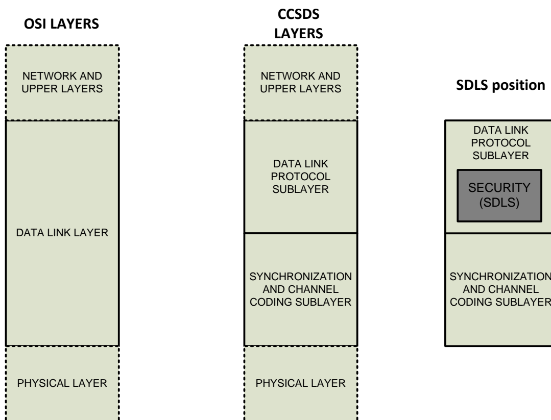
Figure 3-1: OSI vs. CCSDS Layers and SDLS Security Functions Position
