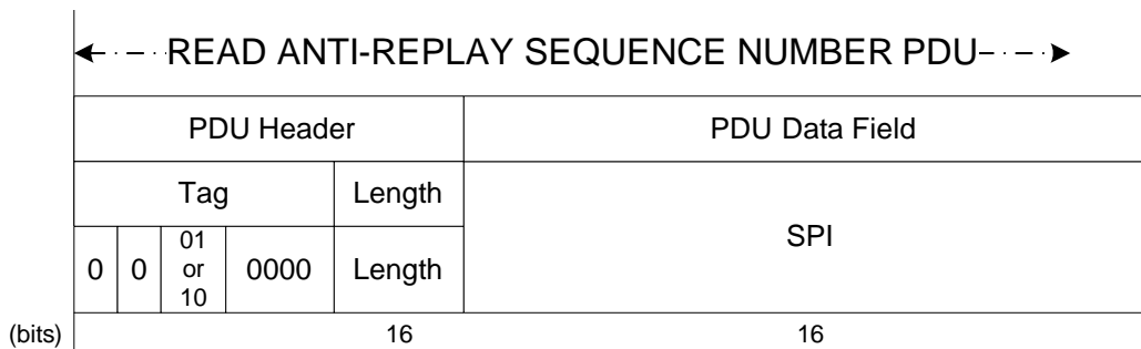
Figure 5-22: Read Anti-Replay Sequence Number Command PDU
