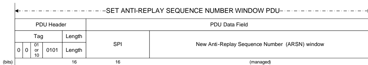
Figure 5-19: Set Anti-Replay Sequence Number Window PDU
