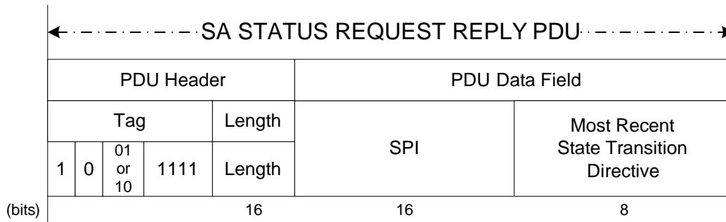
Figure 5-21: SA Status Request Reply PDU
