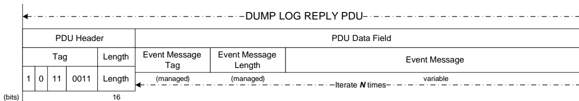
Figure 5-29: Dump Log Reply PDU
