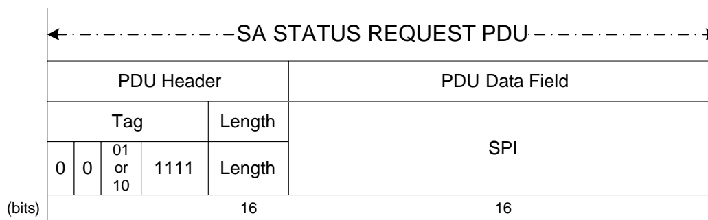
Figure 5-20: SA Status Request PDU
