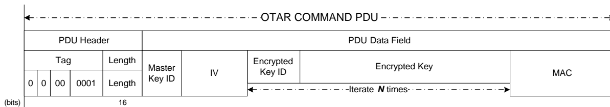
Figure 5-3: OTAR Command PDU
