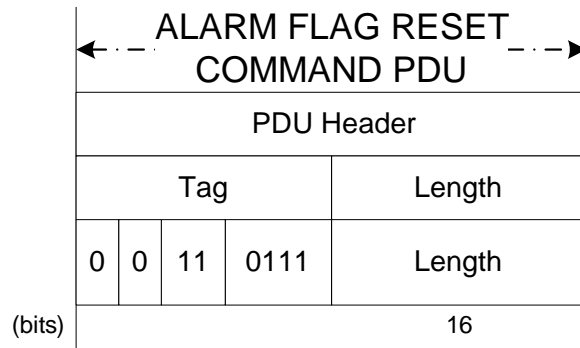
Figure 5-34: Alarm Flag Reset Command PDU
