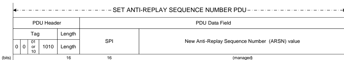
Figure 5-18: Set ARSN PDU
