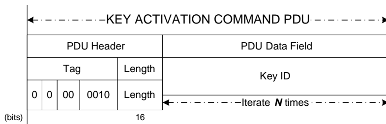
Figure 5-4: Key Activation Command PDU
