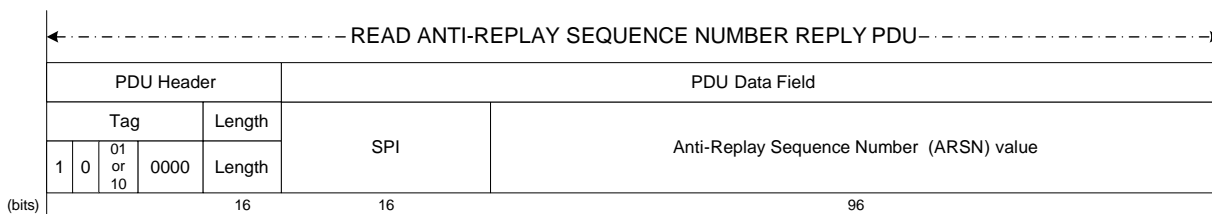
Figure D-12: Read ARSN Reply PDU
