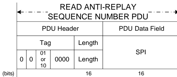
Figure D-11: Read ARSN Command PDU
