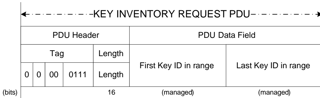
Figure 5-9: Key Inventory Command PDU
