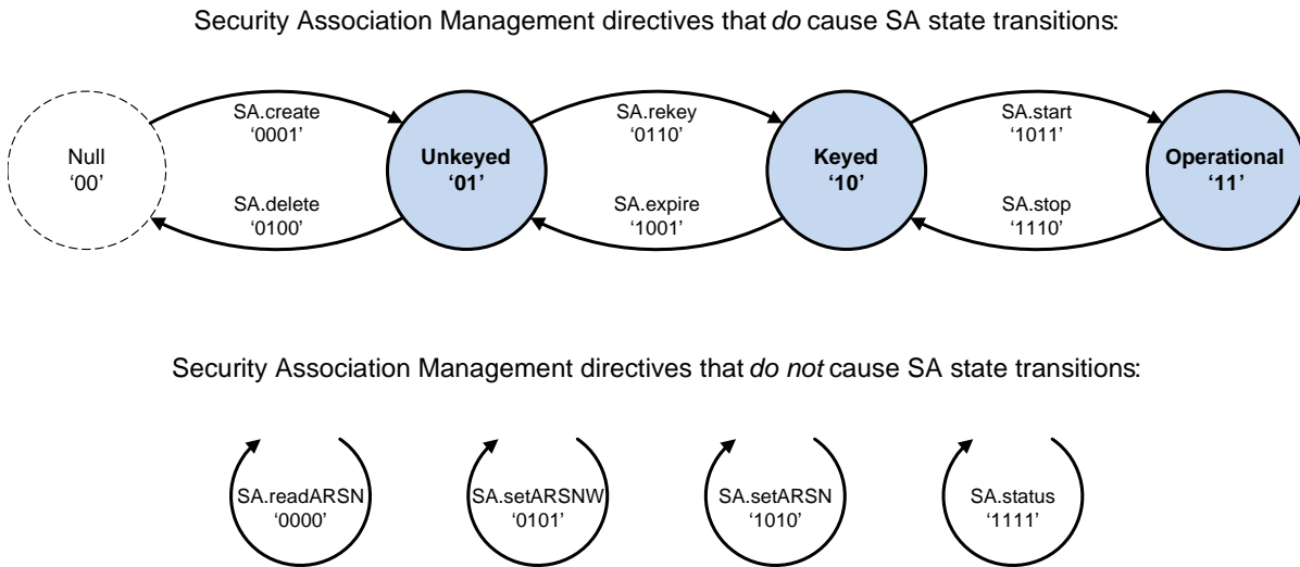
Figure 5-11: SA Management Procedures Overview
