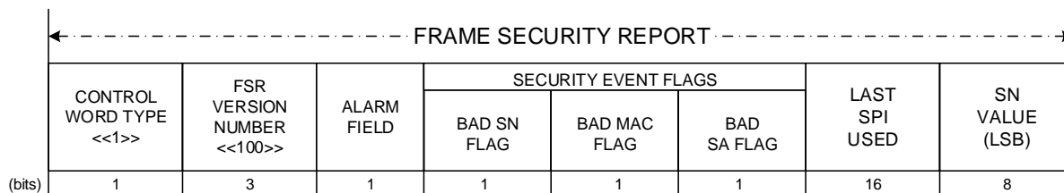
Figure 4-1: Frame Security Report (FSR)
