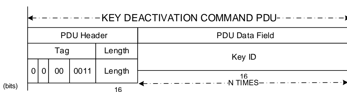
Figure D-3: Baseline Implementation Mode Key Deactivation Command PDU
