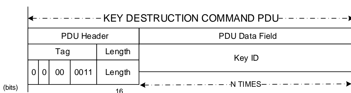
Figure 5-6: Key Destruction Command PDU
