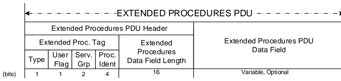
Figure 5-2: Extended Procedures PDU
