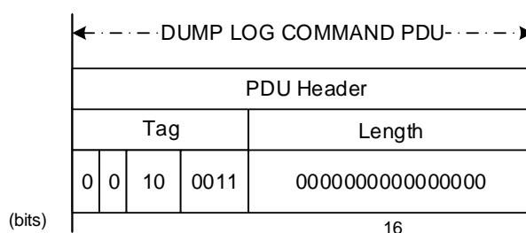
Figure 5-26: Dump Log Command PDU
