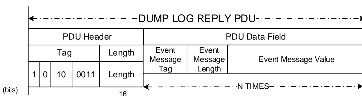
Figure 5-27: Dump Log Reply PDU
