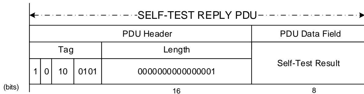
Figure 5-31: Self-Test Reply PDU
