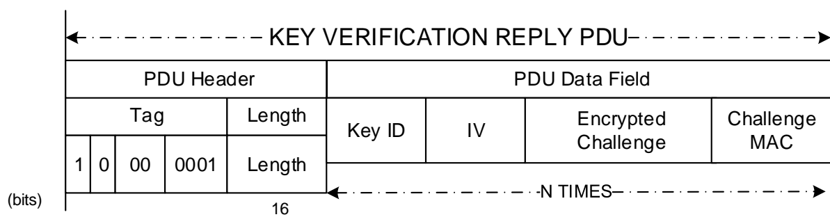
Figure 5-8: Key Verification Reply PDU
