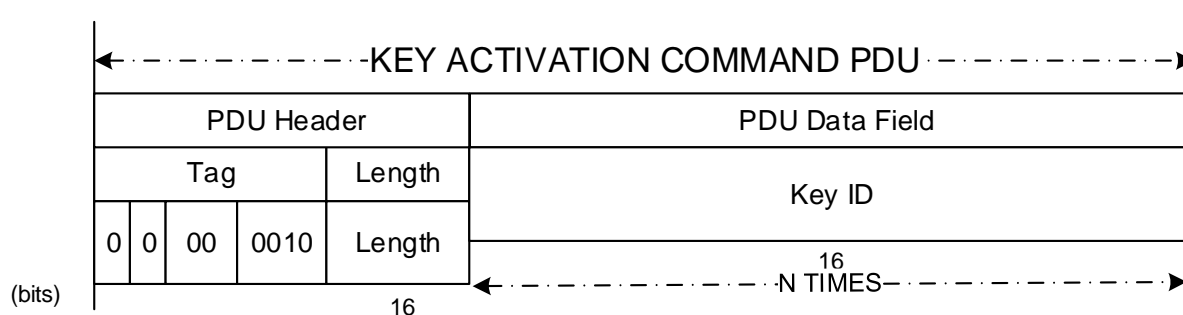
Figure D-2: Baseline Implementation Mode Key Activation Command PDU
