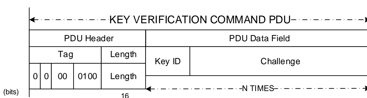
Figure 5-7: Key Verification Command PDU
