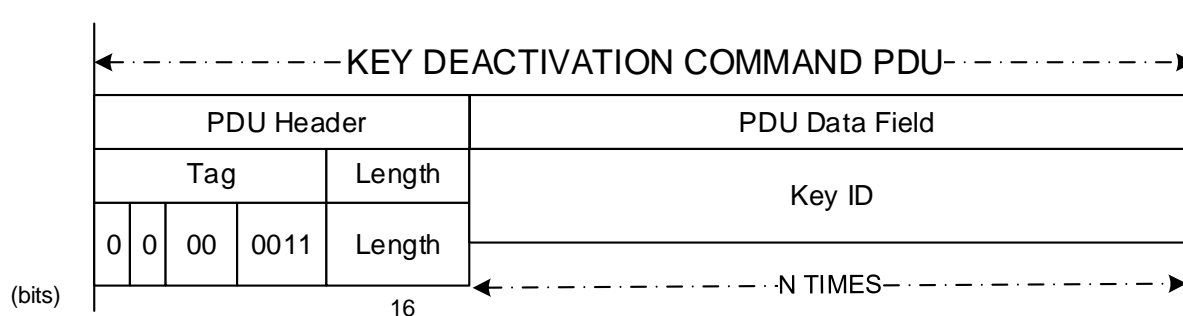
Figure 5-5: Key Deactivation Command PDU
