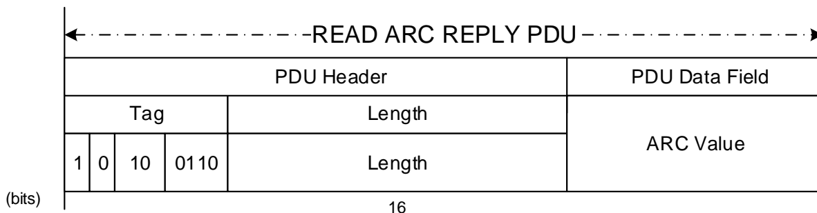
Figure 5-21: Read Sequence Number Reply PDU
