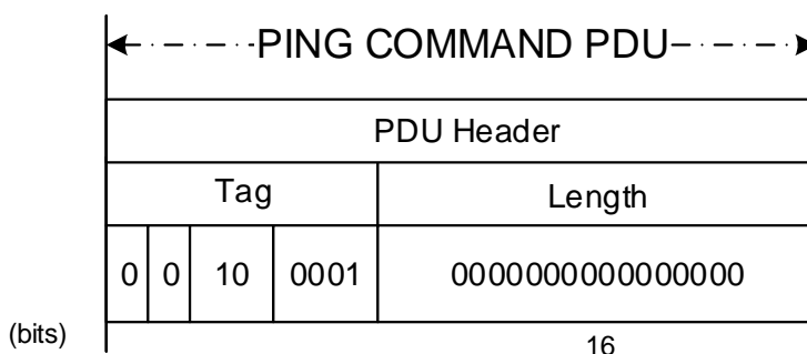
Figure 5-22: Ping Command PDU
