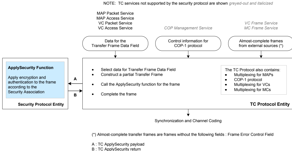
Figure 2-3: Security Protocol Support for TC Services
