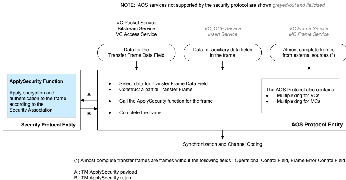
Figure 2-4: Security Protocol Support for AOS Services
