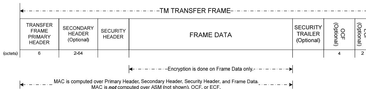
Figure 5-1: TM Transfer Frame Using the Security Protocol
