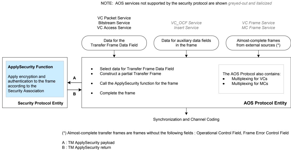
Figure 2-4: Security Protocol Support for AOS Services
