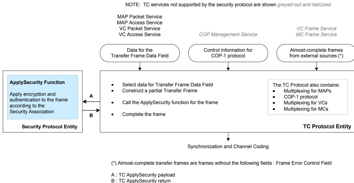
Figure 2-3: Security Protocol Support for TC Services
