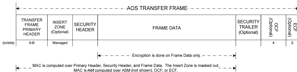
Figure 5-3: AOS Transfer Frame Using the Security Protocol
