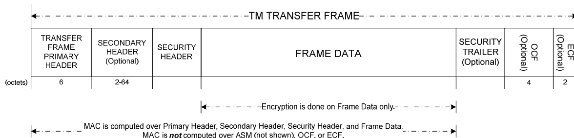
Figure 5-1: TM Transfer Frame Using the Security Protocol
