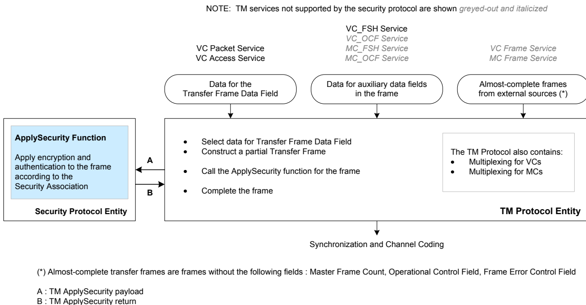
Figure 2-2: Security Protocol Support for TM Services
