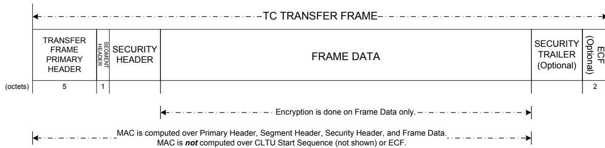
Figure 5-2: TC Transfer Frame Using the Security Protocol
