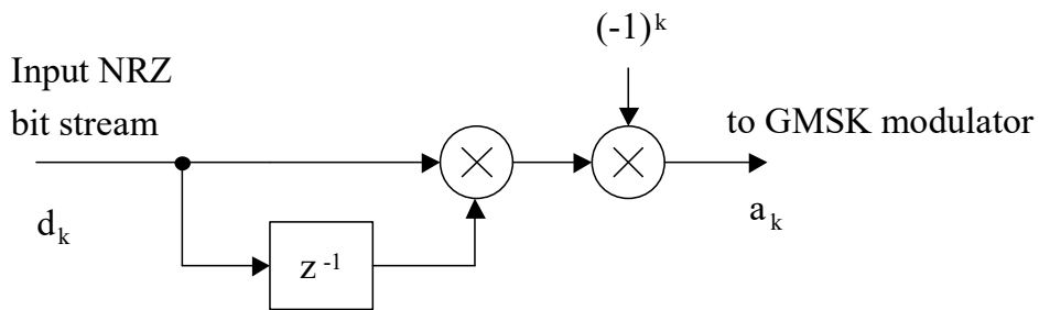
Figure 2.4.25-1: GMSK Precoder
