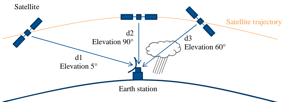
Figure 3-1: Illustration of Variable Conditions of Propagation
