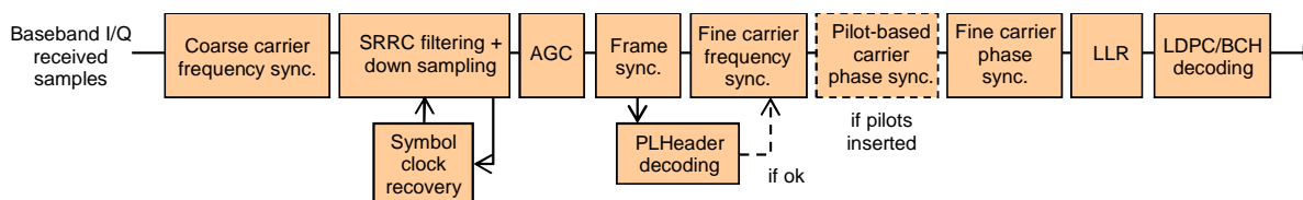
Figure 3-3: Functional Diagram of a Typical DVB-S2 Receiver
