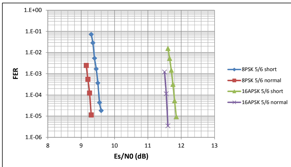
Figure 3-5: DVB-S2 performance with normal and short FECFRAME
