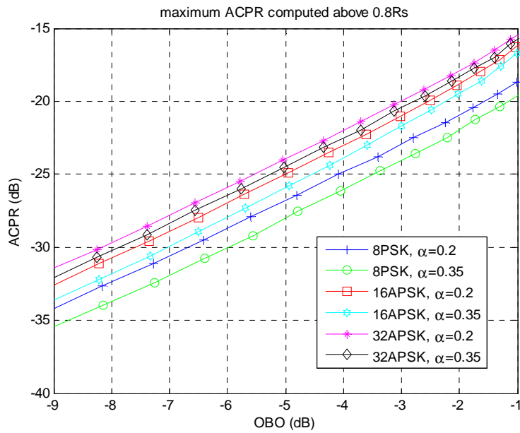
Figure 5- 161615 1615 : ACPR at the PA output
