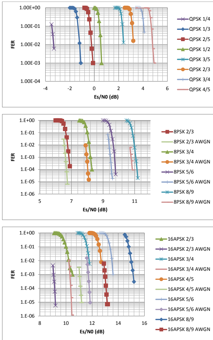
Figure 5-7: Performance with constant |IBO| = 5.5 dB
