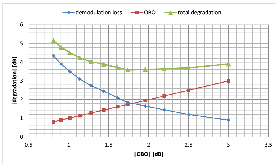
Figure 5-6: Amplifier operating point optimization for 16APSK 8/9
