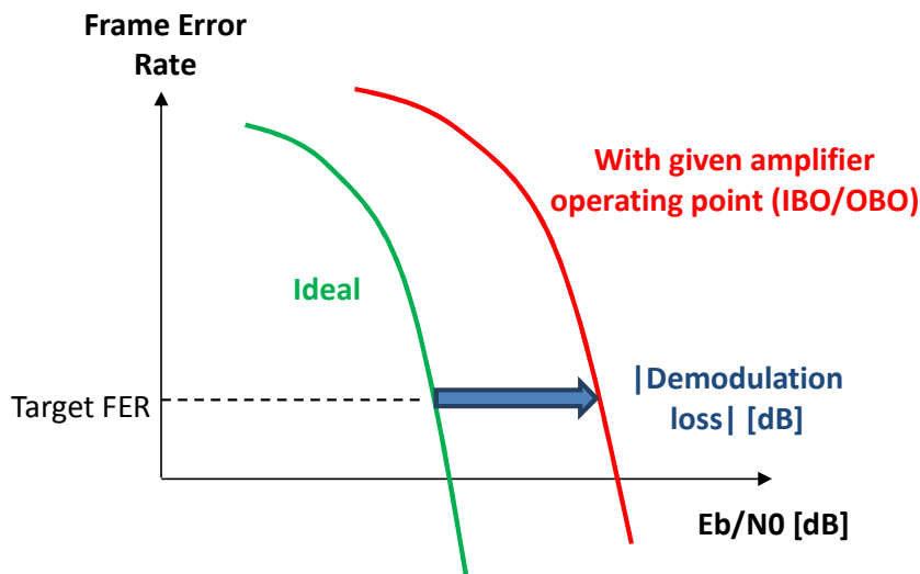
Figure 5-3: DP Principle of demodulation loss measurement principle
