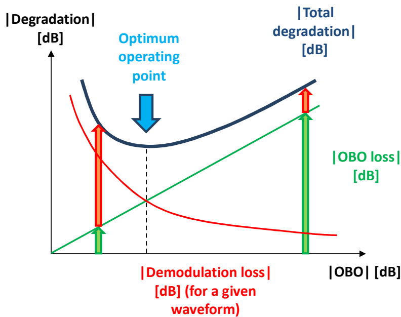
Figure 5-4: Principle of amplifier operating point optimization
