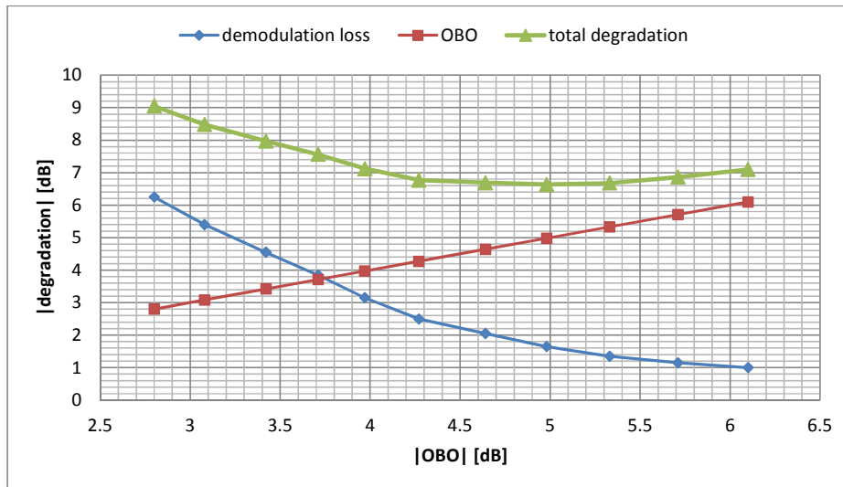
Figure 5-8: Amplifier operating point optimization for 32APSK 8/9
