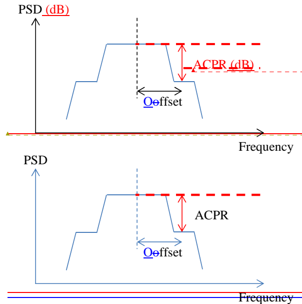
Figure 5-14: Illustration of PAPRACPR measurement
