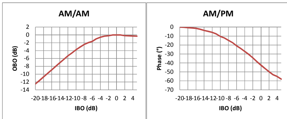
Figure 5-5: 26 GHz power amplifier AM/AM and AM/PM responses
