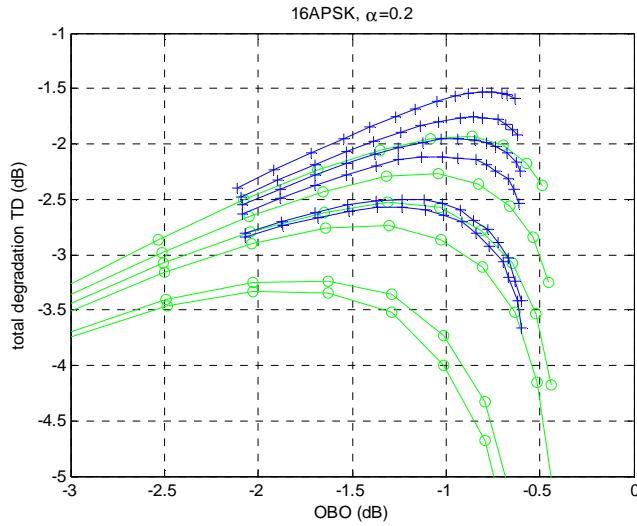
Figure 5-12: Optimal TD for 16APSK
