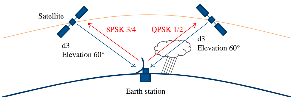
Figure 3-2: Illustration of variable conditions of propagation
