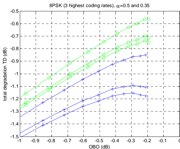
Figure 5-10: TD for 8PSK
