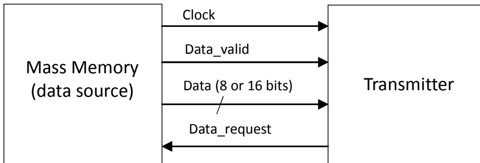
Figure 4-1: Data-pull interface with parallel LVDS wires
