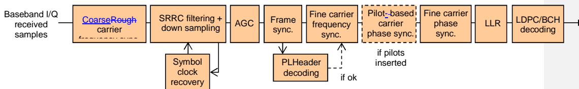
Figure 3-3: Typical DVB-S2 receiver
