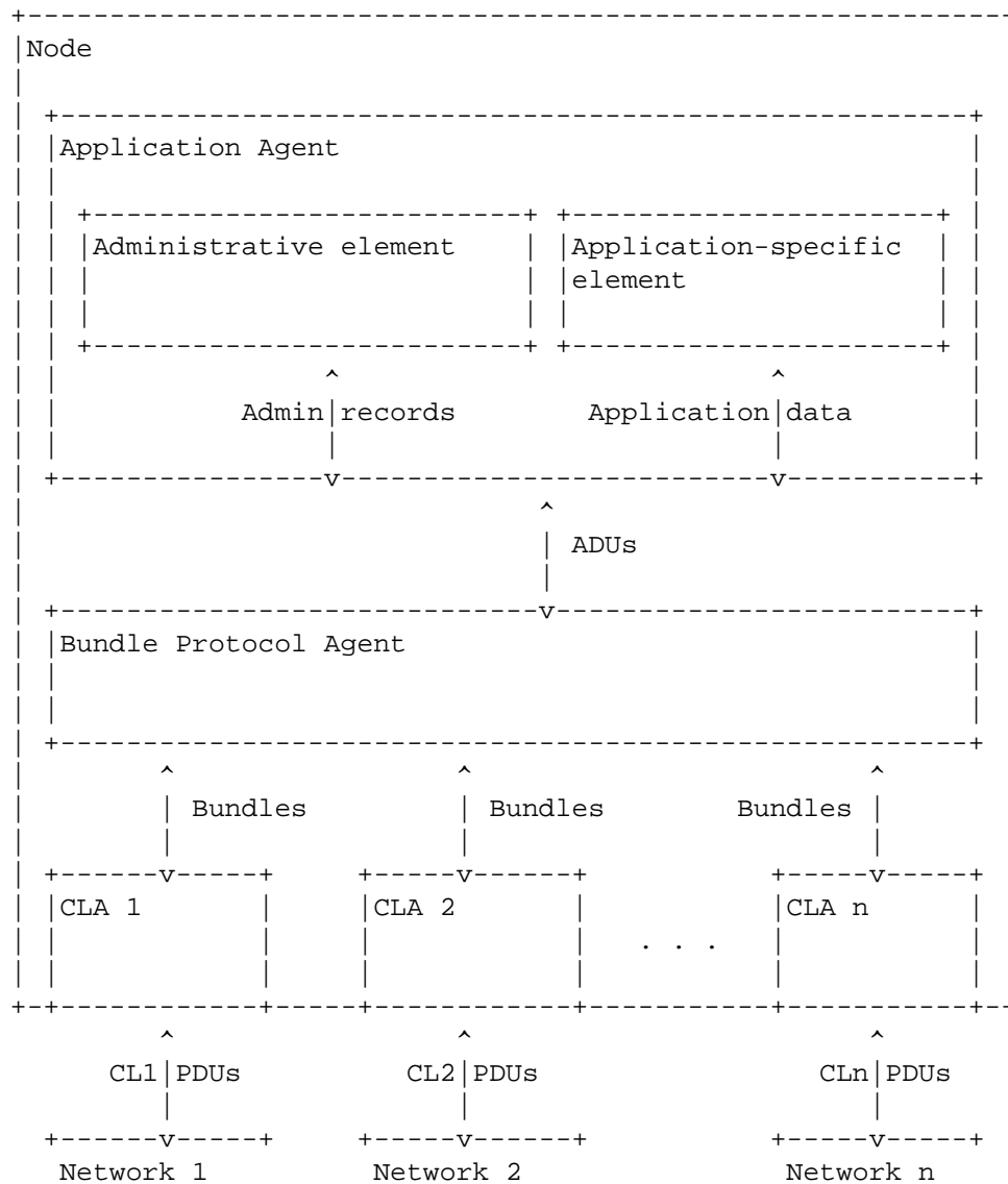
Figure 2: Components of a BP Node
