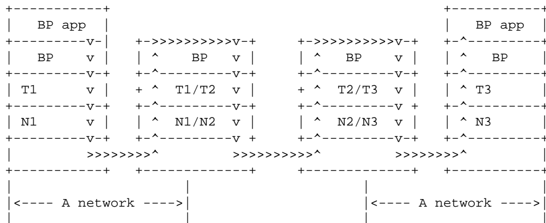
Figure 1: The Bundle Protocol in the Protocol Stack Model
