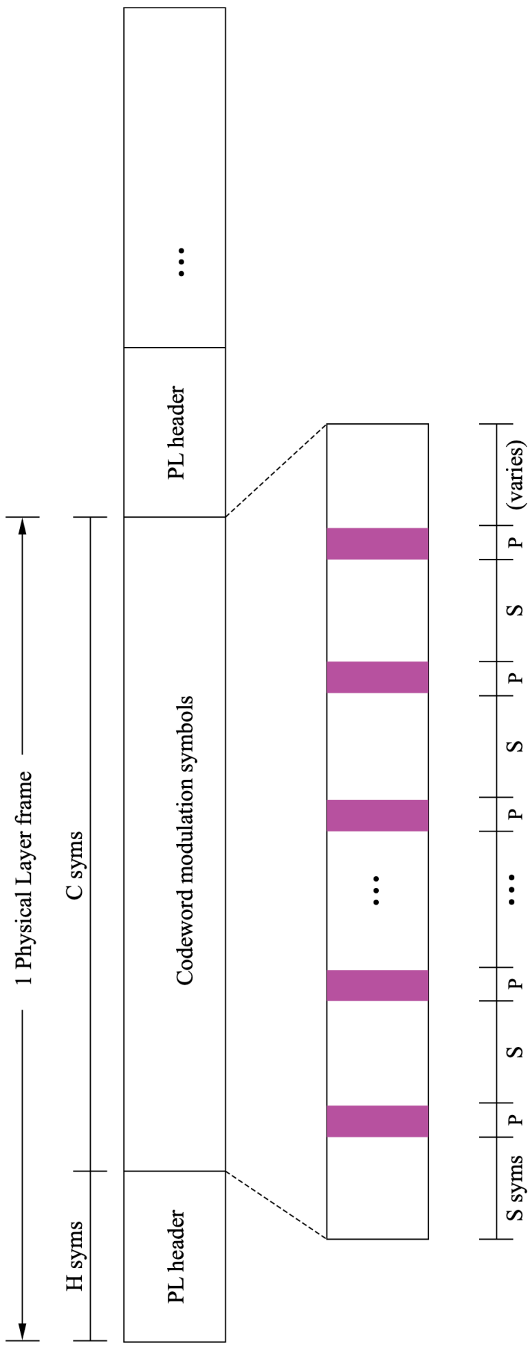
Figure 3-2: Distributed Pilot Pattern
