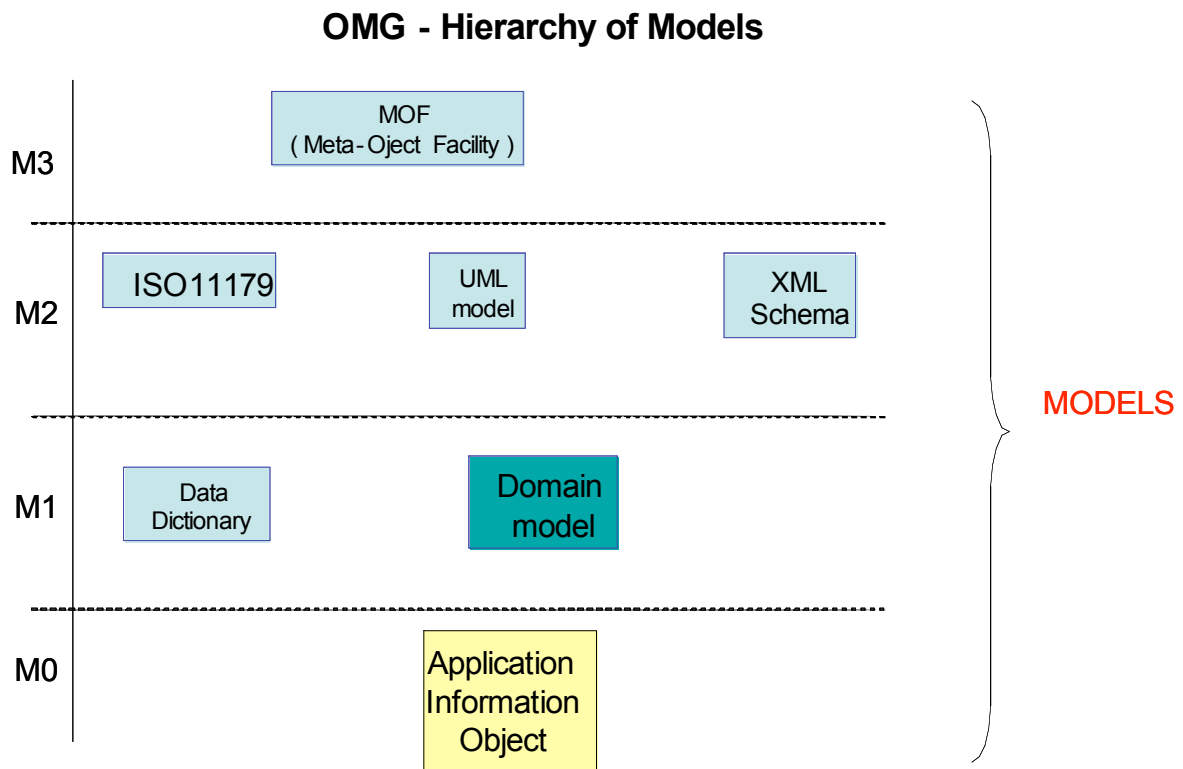
Figure 2-8: Model Hierarchy, Adapted from Reference [24]
