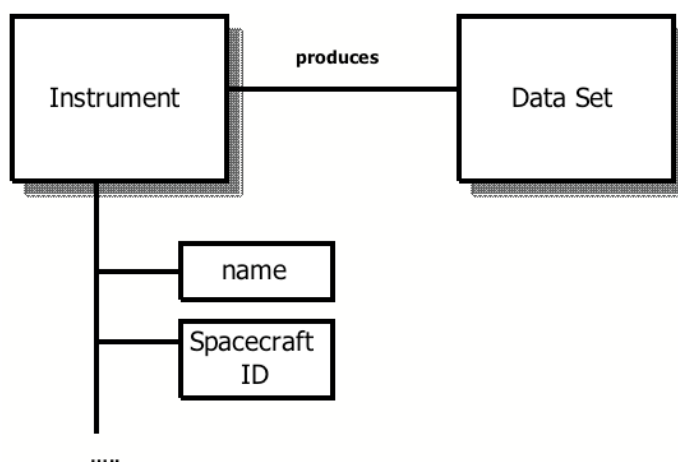
Figure 2-9: Example Planetary Domain Model (Simplified)
