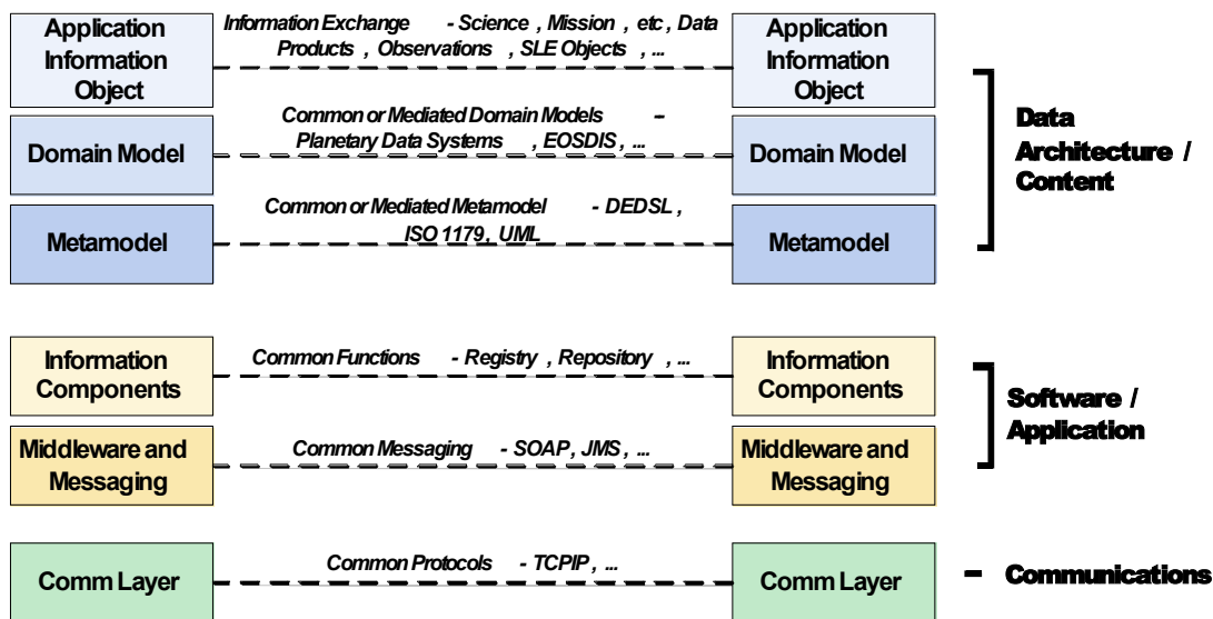
Figure 1-1: High-Level Abstract View of Interoperable Information Architecture
