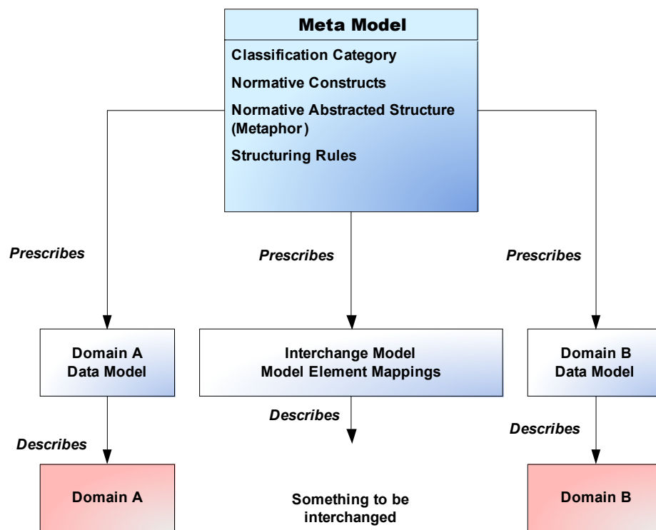
Figure 2-10: Data Models, Meta-Models, and Domains
