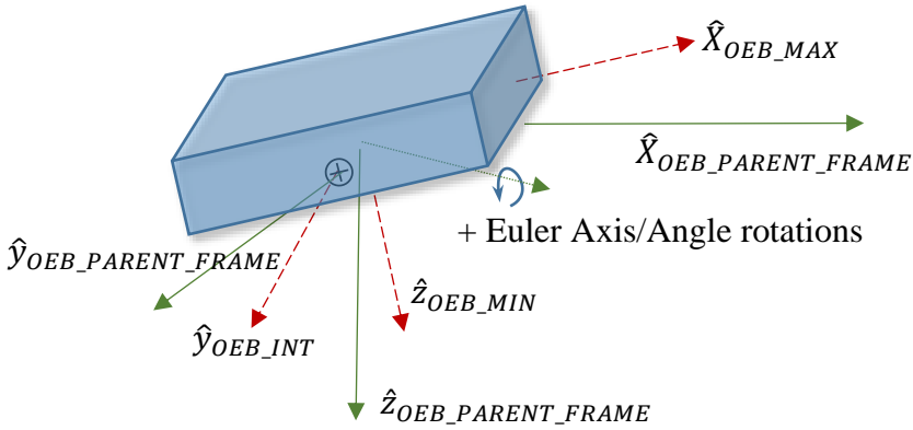
Fig. F- 1 Depiction of Optimally Enclosing Box and definitions of MAX, INT, and MIN orientation vectors relative to OEB parent frame
