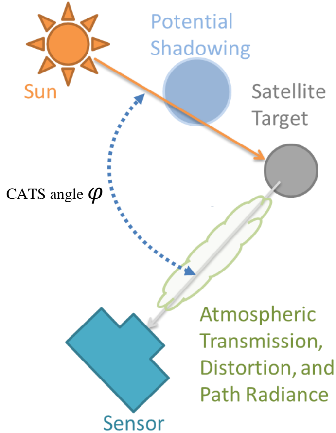
Fig. F- 2 Depiction of optical viewing Critical Angle to the Sun (CATS) angle geometry
