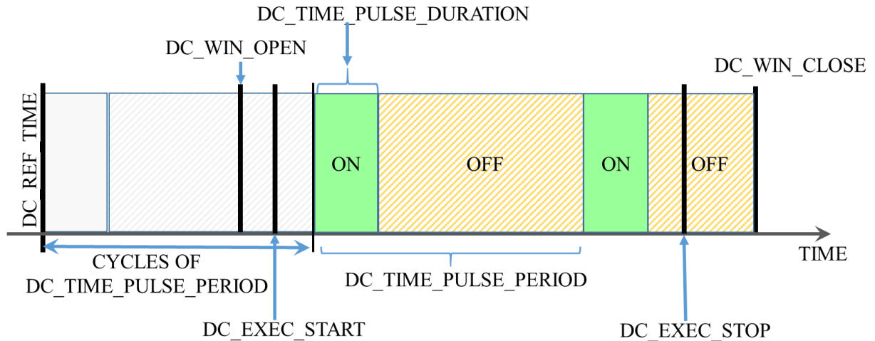
Fig. F-3 Diagram of time-based duty cycle ( DC\_TYPE = "TIME" )
