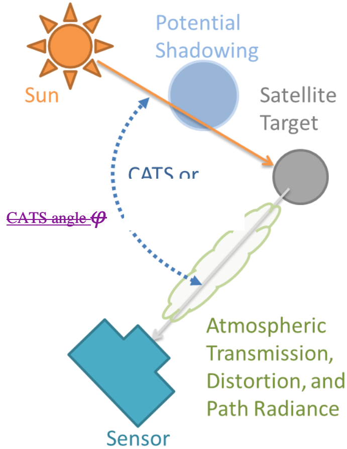
Fig. E-F-2 Depiction of optical viewing Critical Angle to the Sun (CATS) angle geometry
