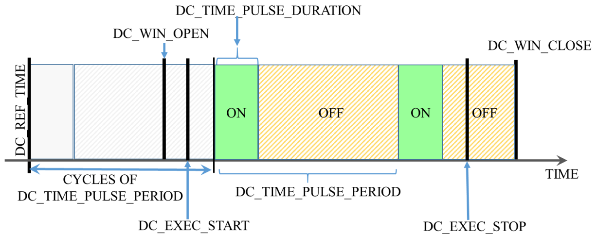
Fig. C- 3 Diagram of time-based duty cycle ( DC\_TYPE = "TIME" )
