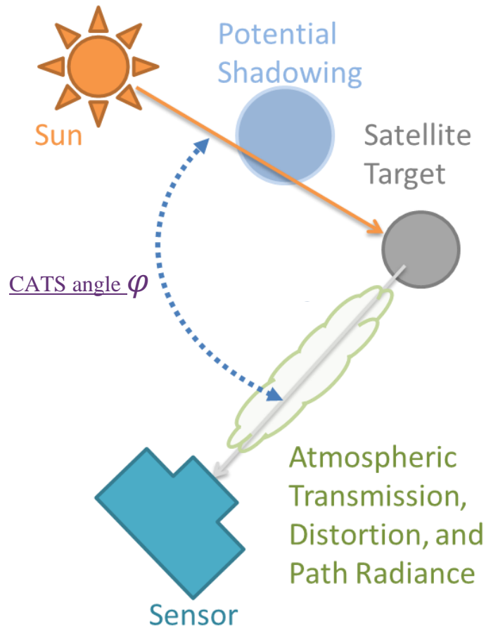
Fig. C-2 Depiction of optical viewing Critical Angle to the Sun (CATS) phase -angle geometry
