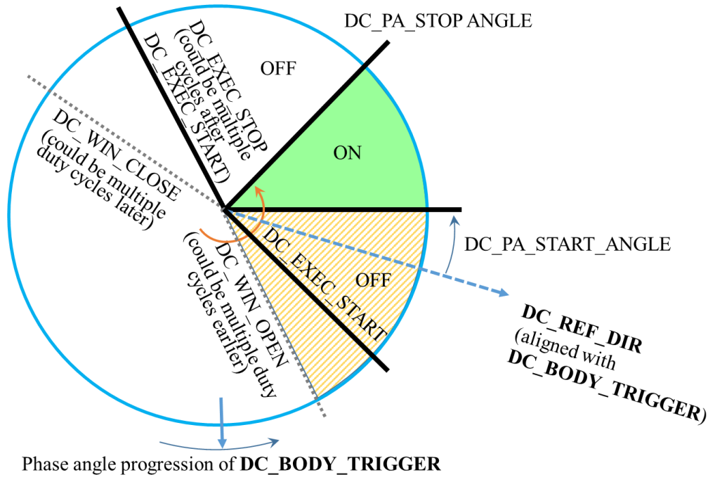
Fig. C-4 Diagram of a rotating spacecraft body's progression through an inertial clock angle-based duty cycle ( DC\_TYPE = "TIME\_AND\_ANGLE" )
