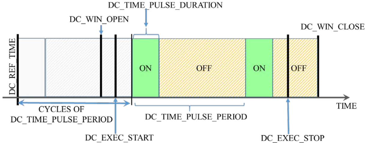
Fig. C- 3 Diagram of time-based duty cycle (DC_TYPE = "TIME")
