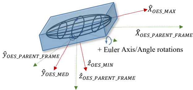
Fig. C- 1 Depiction of BOX and ELLIPSOID shape type and definitions of MAX, MED and MIN orientation vectors relative to OES parent frame
