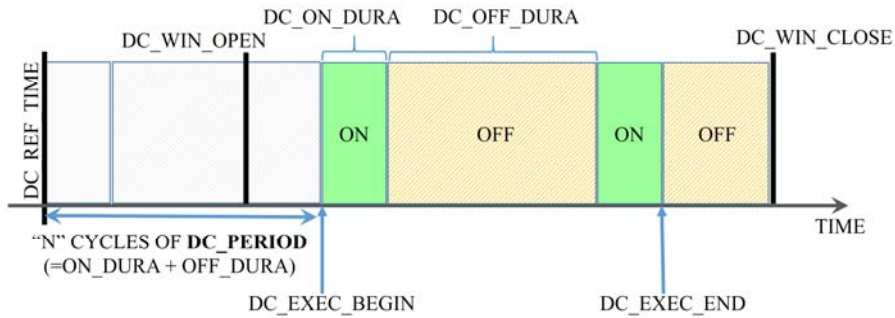
Fig. C- 4 Diagram of time-based duty cycle ( MAN_DUTY_CYCLE_TYPE = “TIME”)
