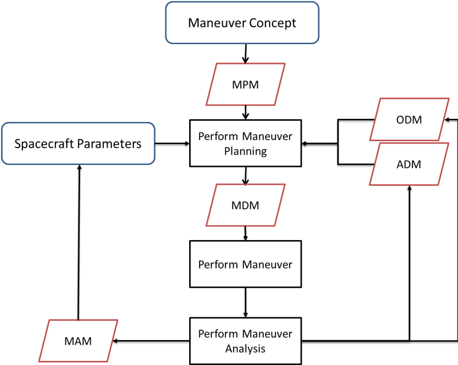
Figure 4-6: SMM, ODM and ADM Use Case Example
