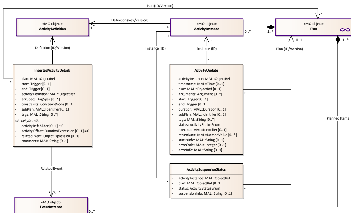
Figure 3-6: Activity Service Structures
