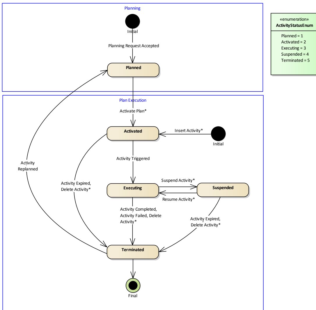
Figure 3-4: Activity State Model
