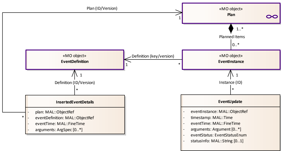
Figure 3-9: Event Service Structures
