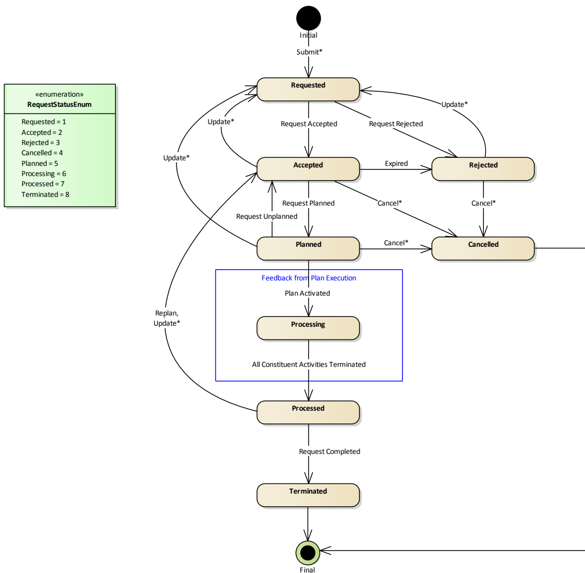
Figure 3-14: Planning Request State Model
