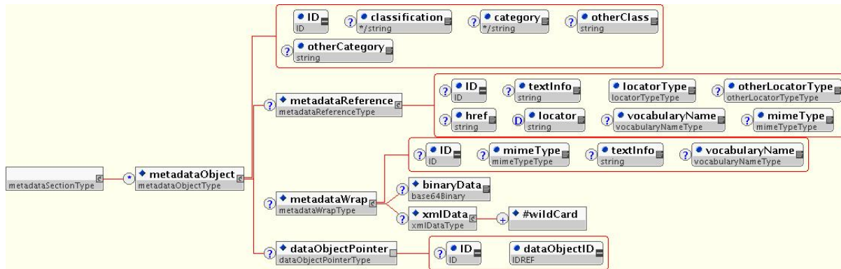
Figure 9-1: metadataObjectType and metadataSectionType Schema Diagram
