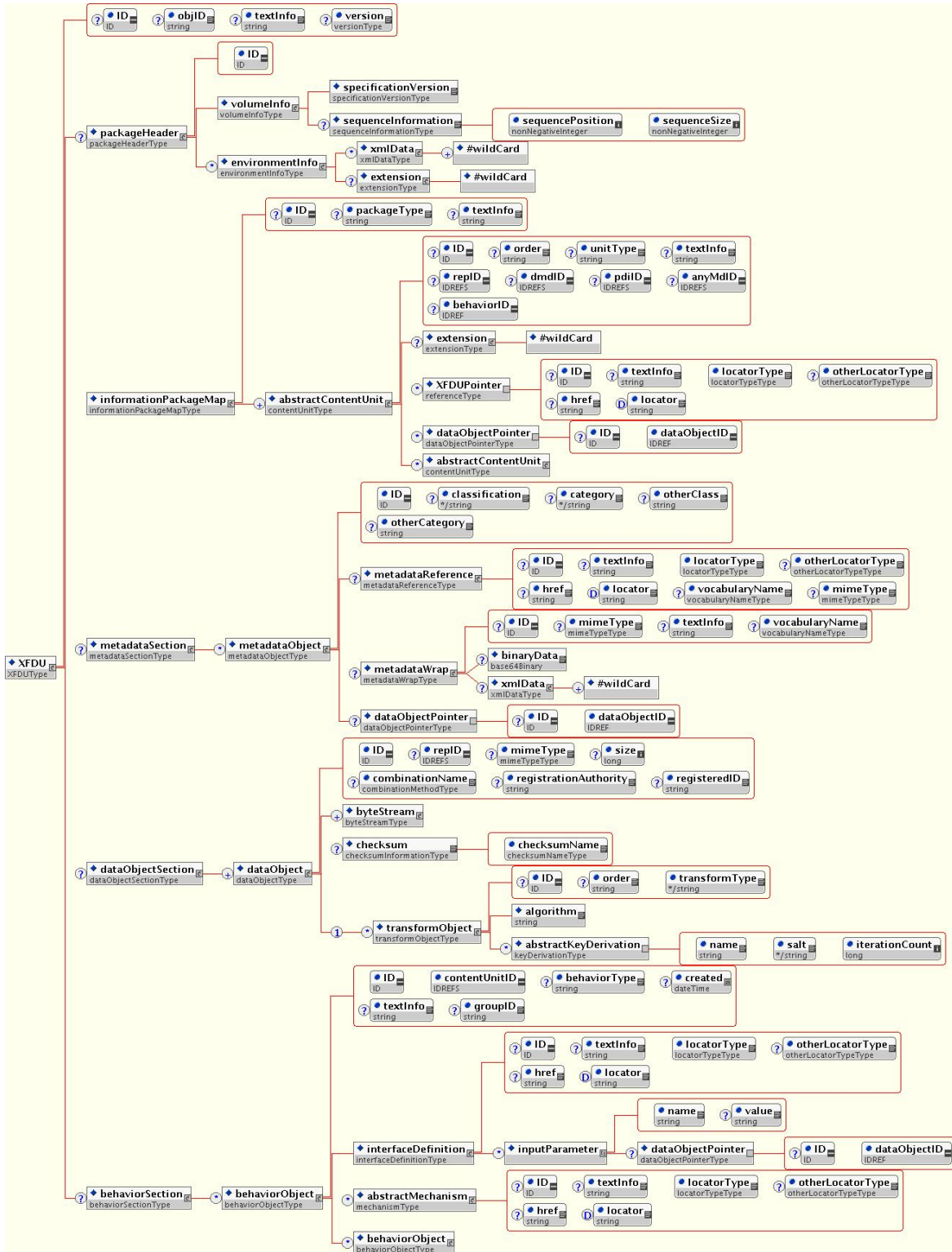
Figure 11-1: Full XFDU Schema Diagram
