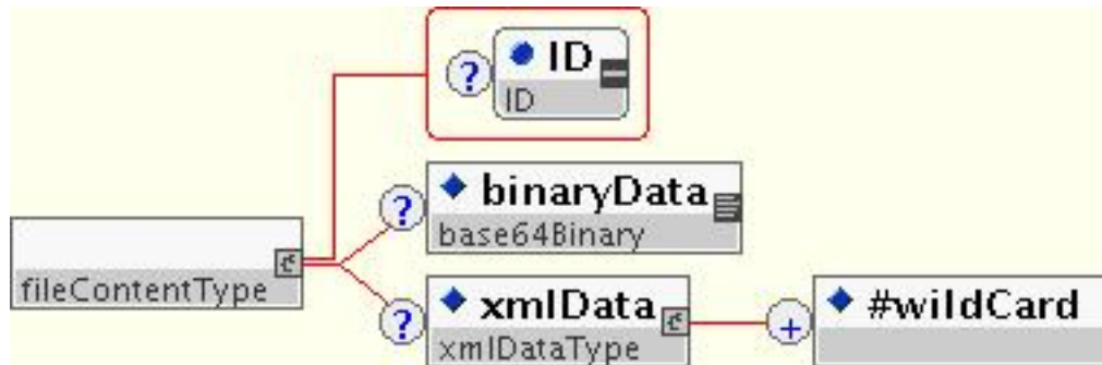
Figure 4-5: fileContentType/binaryData/xmlData 1 Schema Diagram
