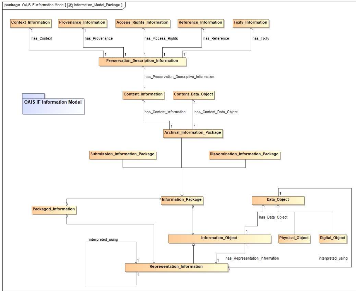
Figure 13 - OAIS Information Model
